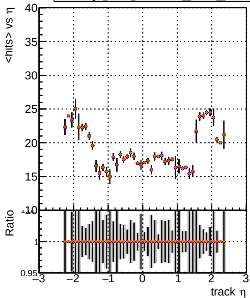
mean hit DQM_V0001_R000000001 Global CMSSW_orig DQM_V0001_R000000001 Global CMSSW_pl08 DQM_V0001_R000000001 Global CMSSW_pl075 DQM_V0001_R000000001 Global CMSSW_pl07
