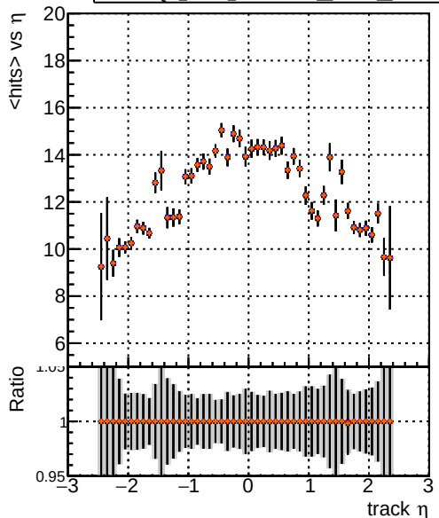
mean hits DQM_V0001_R000000001 Global CMSSW_orig DQM_V0001_R000000001 Global CMSSW_pl08 DQM_V0001_R000000001 Global CMSSW_pl075 DQM_V0001_R000000001 Global CMSSW_pl07
