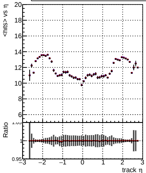
mean hits DQM_V0001_R000000001_Global_CMSSW_orig DQM_V0001_R000000001_Global_CMSSW_hpt08 DQM_V0001_R000000001_Global_CMSSW_hpt05
