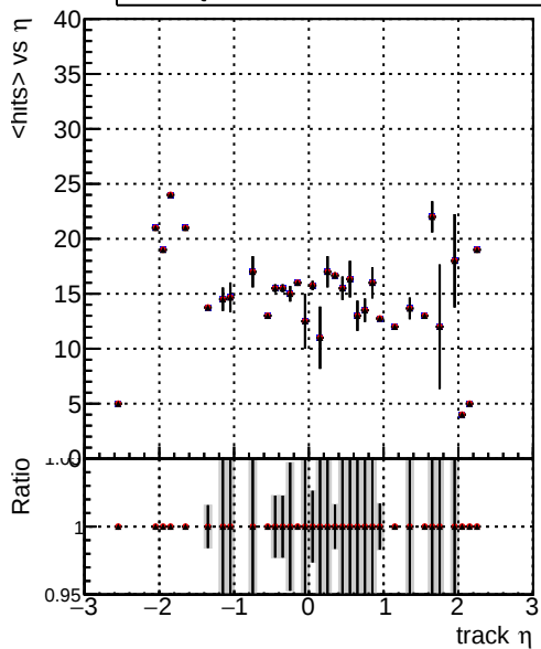
mean hits DQM_V0001_R000000001_Global_CMSSW_orig DQM_V0001_R000000001_Global_CMSSW_hpt08 DQM_V0001_R000000001_Global_CMSSW_hpt05
