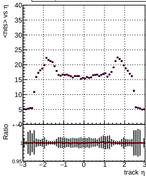
mean hits vs \eta DQM_V0001_R000000001_Global_CMSSW_orig DQM_V0001_R000000001_Global_CMSSW_hpt08 DQM_V0001_R000000001_Global_CMSSW_hpt05
