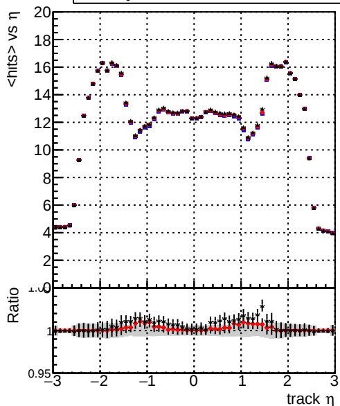
mean hits vs \eta DQM_V0001_R000000001_Global_CMSSW_orig DQM_V0001_R000000001_Global_CMSSW_hpt08 DQM_V0001_R000000001_Global_CMSSW_hpt05
