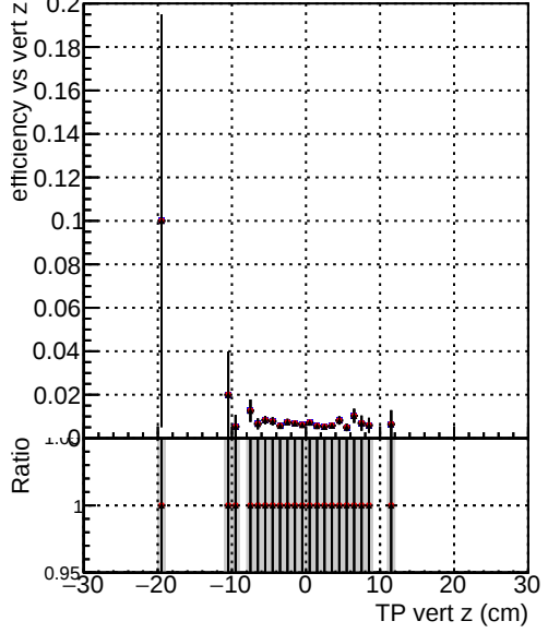
Efficiency vs. TP vert z (cm) —●— DQM_V0001_R0000000001_Global_CMSSW_orig —●— DQM_V0001_R0000000001_Global_CMSSW_hpt08 —●— DQM_V0001_R0000000001_Global_CMSSW_hpt05
