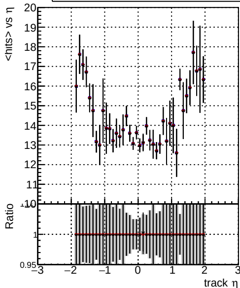
mean hit DQM_V0001_R0000000001_Global_CMSSW_orig DQM_V0001_R0000000001_Global_CMSSW_hpt08 DQM_V0001_R0000000001_Global_CMSSW_hpt05
