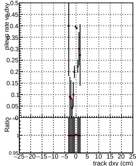
Global CMSSW hbt08
