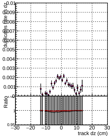
Global CMSSW orig
