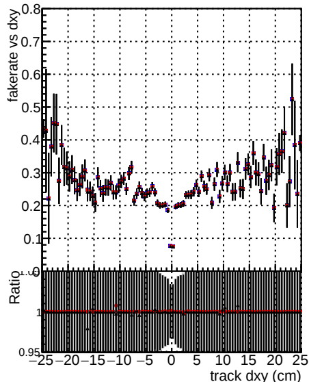
DOM V0001 R0000000001 Global CMSSW orig DOM V0001 R0000000001 Global CMSSW hbt08
