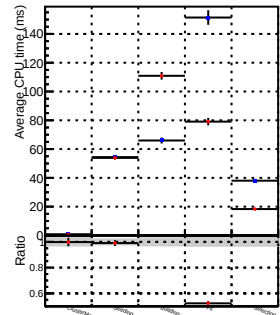
highPTripletStep
