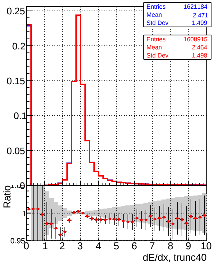
DQM_V0001_R000000001_Global_CMSSW_orig DQM_V0001_R000000001_Global_mkFitALLCHA_RECO
