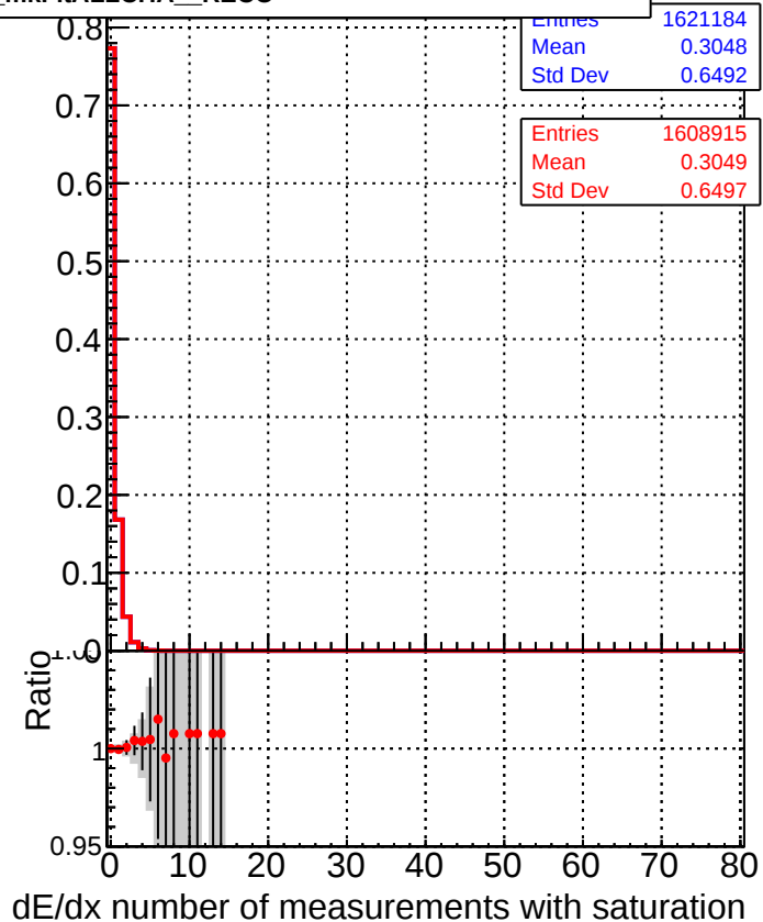
DQM_V0001_R000000001_Global_CMSSW_orig DQM_V0001_R000000001_Global_mkFitALLCHA_RECO
