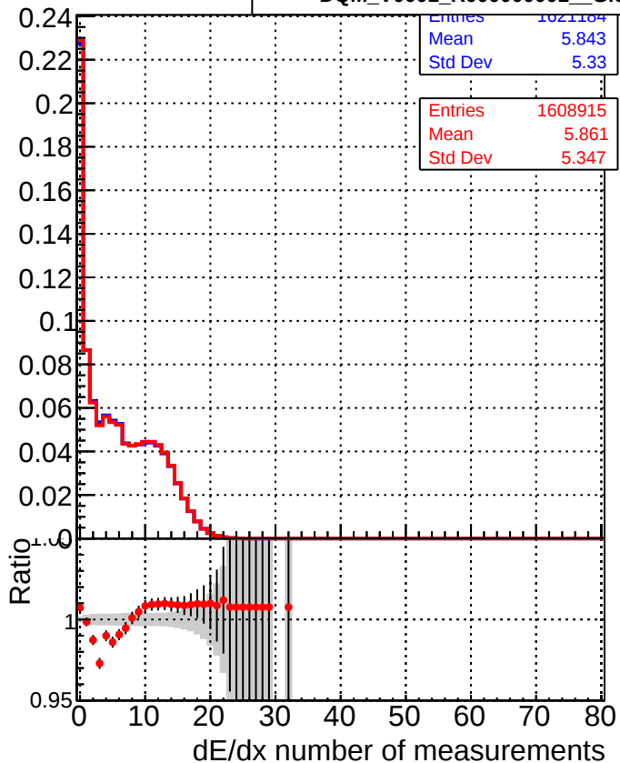
DQM_V0001_R000000001_Global_CMSSW_orig DQM_V0001_R000000001_Global_mkFitALLCHA_RECO
