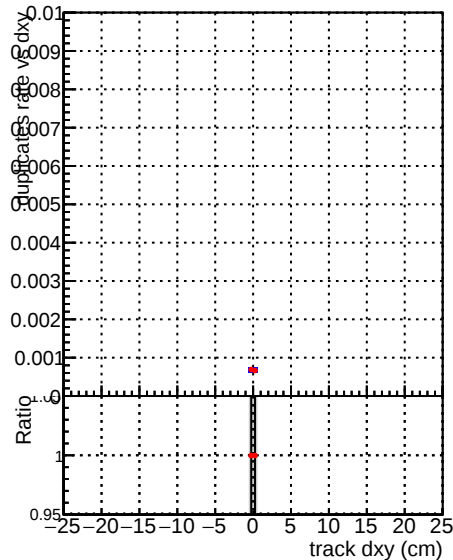
al__CMSSW_orig al__mkFitALLCHA__RECO
