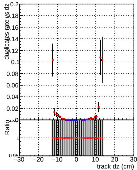
al__CMSSW_orig al__mkFitALLCHA__RECO
