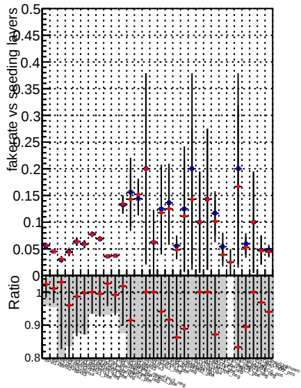
Fake rate vs. —●— DQM V0001_R000000001 Global CMSSW_orig —●— DQM V0001_R000000001 Global mkFitALLCHA RECO
