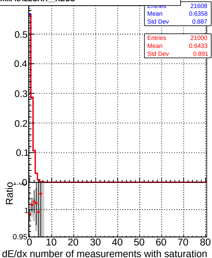
DQM_V0001_R000000001_Global_CMSSW_orig DQM_V0001_R000000001_Global_mkFitALLCHA_RECO
