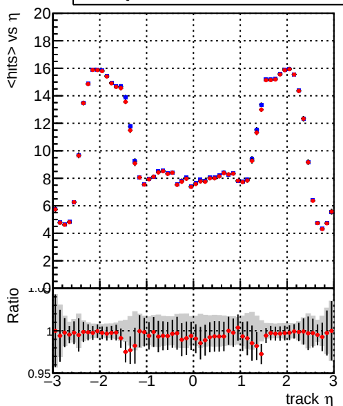
— DQM_V0001_R000000001_Global_CMSSW_orig — DQM_V0001_R000000001_Global_mkFitALLCHA_RECO
