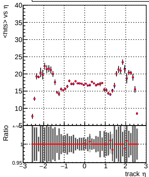
mean hit — DQM_V0001_R000000001_Global_CMSSW_orig — DQM_V0001_R000000001_Global_mkFitALLCHA_RECO
