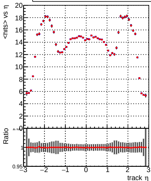
mean hit — DQM_V0001_R000000001_Global_CMSSW_orig — DQM_V0001_R000000001_Global_mkFitALLCHA_RECO
