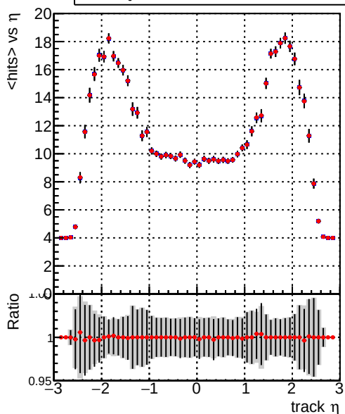
— DQM_V0001_R000000001_Global_CMSSW_orig — DQM_V0001_R000000001_Global_mkFitALLCHA_RECO
