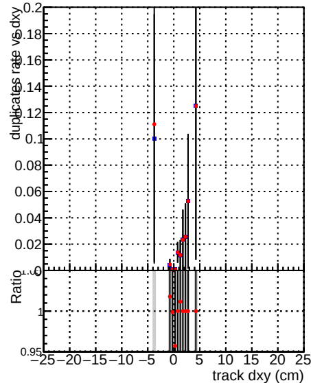
al_CMSSW_orig al_mkFitALLCHA_RECO 0 0.987 0.986 1 0.987 0.986 2 0.987 0.986 3 0.987 0.986 4 0.987 0.986 5 0.987 0.986 6 0.987 0.986 7 0.987 0.986 8 0.987 0.986 9 0.987 0.986 10 0.987 0.986 11 0.987 0.986 12 0.987 0.986 13 0.987 0.986 14 0.987 0.986 15 0.987 0.986 16 0.987 0.986 17 0.987 0.986 18 0.987 0.986 19 0.987 0.986 20 0.987 0.986 21 0.987 0.986 22 0.987 0.986 23 0.987 0.986 24 0.987 0.986 25 0.987 0.986 26 0.987 0.986 27 0.987 0.986 28 0.987 0.986 29 0.987 0.986 30 0.987 0.986 31 0.987 0.986 32 0.987 0.986 33 0.987 0.986 34 0.987 0.986 35 0.987 0.986 36 0.987 0.986 37 0.987 0.986 38 0.987 0.986 39 0.987 0.986 40 0.987 0.986 41 0.987 0.986 42 0.987 0.986 43 0.987 0.986 44 0.987 0.986 45 0.987 0.986 46 0.987 0.986 47 0.987 0.986 48 0.987 0.986 49 0.987 0.986 50 0.987 0.986 51 0.987 0.986 52 0.987 0.986 53 0.987 0.986 54 0.987 0.986 55 0.987 0.986 56 0.987 0.986 57 0.987 0.986 58 0.987 0.986 59 0.987 0.986 60 0.987 0.986 61 0.987 0.986 62 0.987 0.986 63 0.987 0.986 64 0.987 0.986 65 0.987 0.986 66 0.987 0.986 67 0.987 0.986 68 0.987 0.986 69 0.987 0.986 70 0.987 0.986 71 0.987 0.986 72 0.987 0.986 73 0.987 0.986 74 0.987 0.986 75 0.987 0.986 76 0.987 0.986 77 0.987 0.986 78 0.987 0.986 79 0.987 0.986 80 0.987 0.986 81 0.987 0.986 82 0.987 0.986 83 0.987 0.986 84 0.987 0.986 85 0.987 0.986 86 0.987 0.986 87 0.987 0.986 88 0.987 0.986 89 0.987 0.986 90 0.987 0.986 91 0.987 0.986 92 0.987 0.986 93 0.987 0.986 94 0.987 0.986 95 0.987 0.986 96 0.987 0.986 97 0.987 0.986 98 0.987 0.986 99 0.987 0.986
