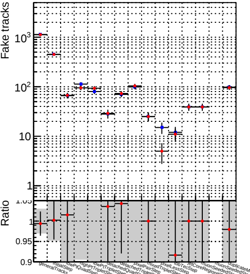
Number —●— DQM_V0001_R0000000001_Global_mkFitALLCHA_RECO
