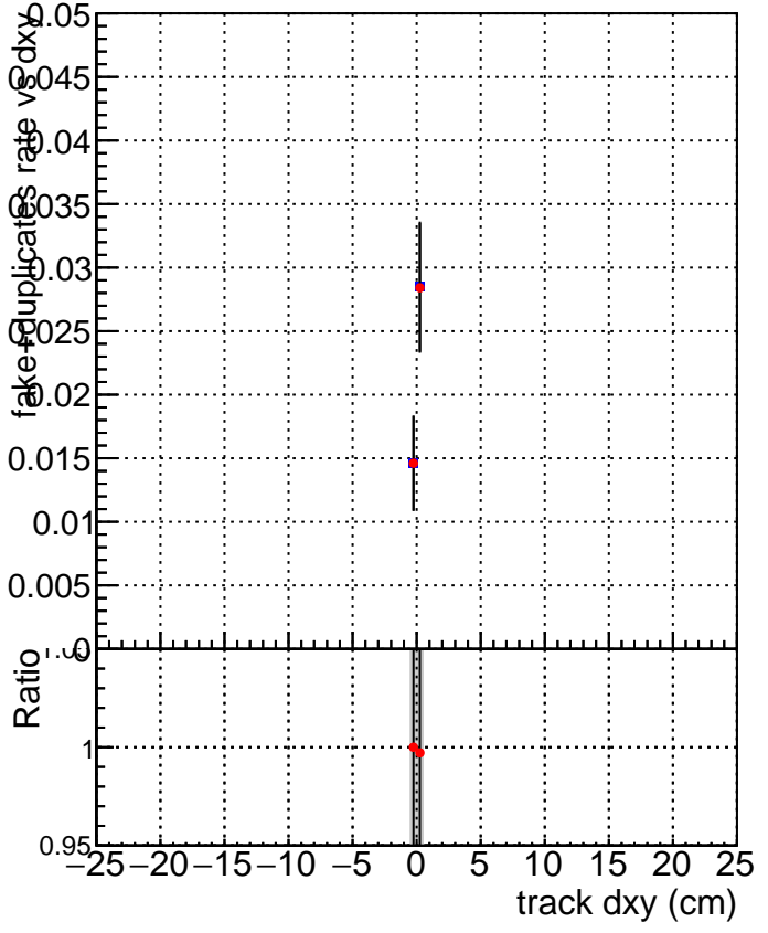
DQM_V0001_R000000001_Global_CMSSW_orig DQM_V0001_R000000001_Global_mkFitALLCHA_RECO
