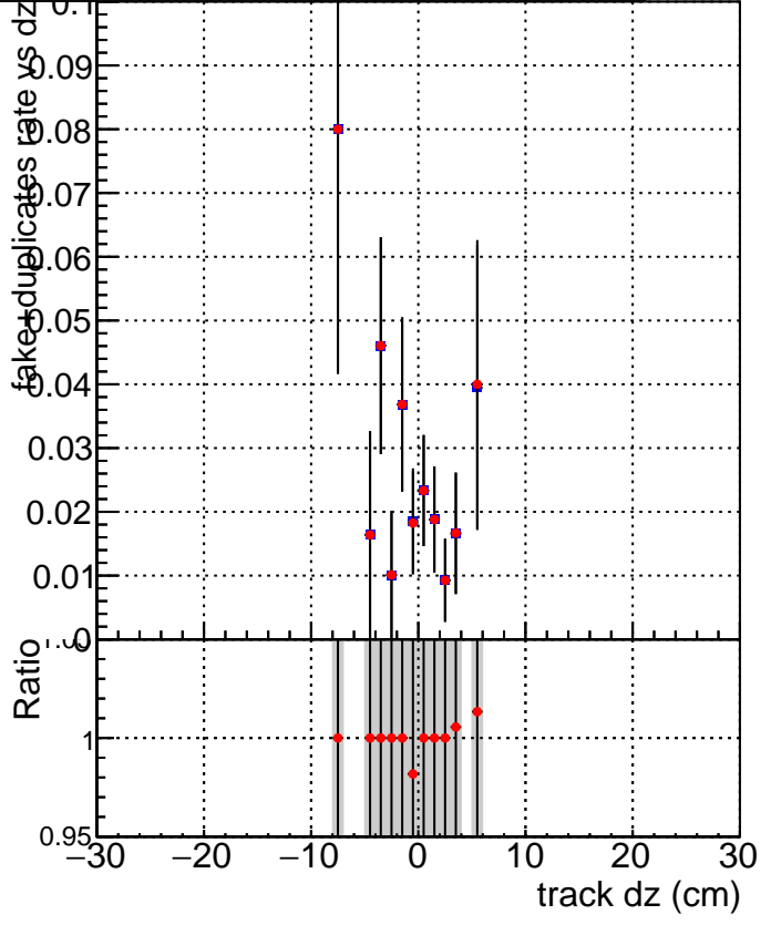
DQM_V0001_R000000001_Global_CMSSW_orig DQM_V0001_R000000001_Global_mkFitALLCHA_RECO
