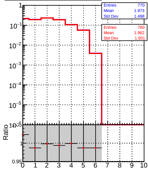
— DQM_V0001_R000000001_Global_CMSSW_orig — DQM_V0001_R000000001_Global_mkFitALLCHA_RECO
