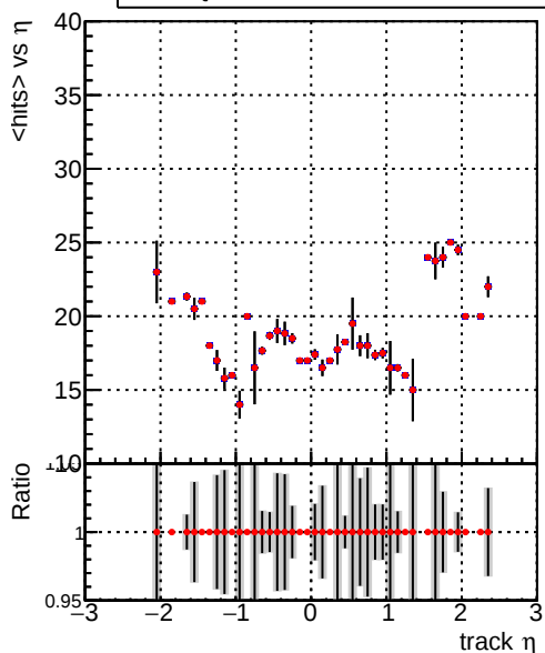
mean hit — DQM_V0001_R000000001_Global_CMSSW_orig — DQM_V0001_R000000001_Global_mkFitALLCHA_RECO
