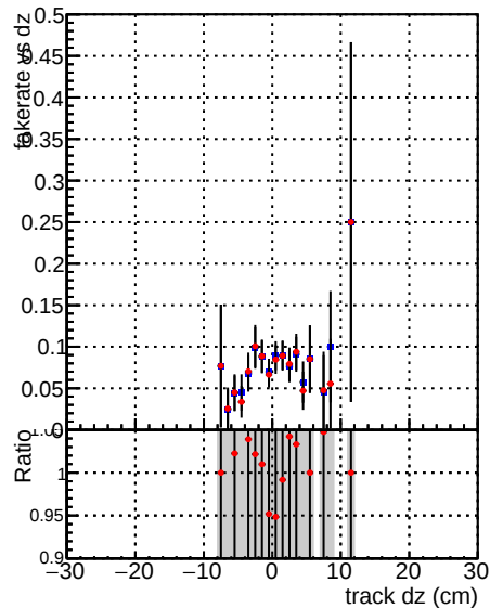
Global CMSSW_orig —●— DQM_V0001_R0000000001 Global mkFitALLCHA RECO —●— DQM_V0001_R0000000001 Global mkFitALLCHA RECO
