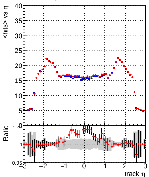
mean hits — DQM_V0001_R000000001_Global_CMSSW_orig — DQM_V0001_R000000001_Global_mkFitALLCHA_RECO
