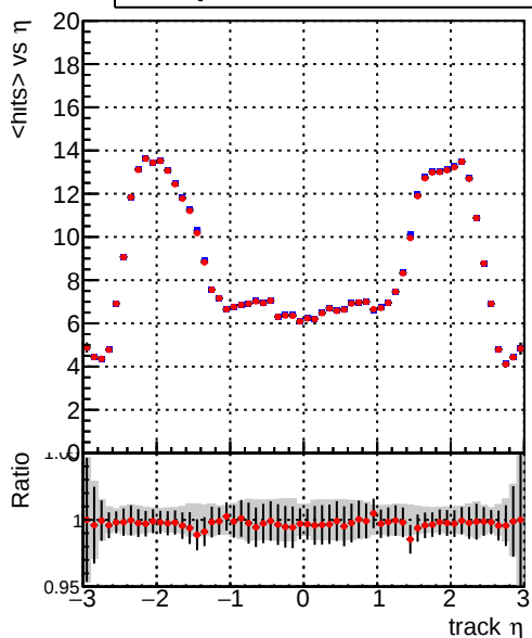
mean hits vs \eta — DQM_V0001_R000000001_Global_CMSSW_orig — DQM_V0001_R000000001_Global_mkFitALLCHA_RECO
