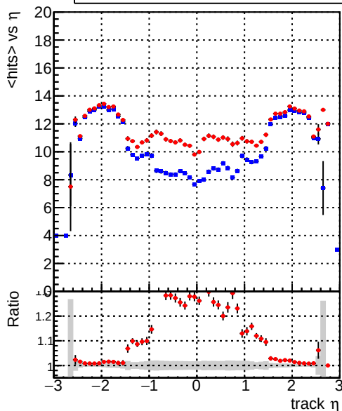
DQM_V0001_R000000001_Global_CMSSW_orig mean hits DQM_V0001_R000000001_Global_mkFitALLCHA_RECO
