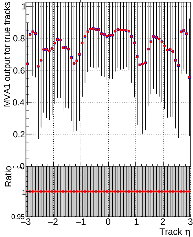
MVA1 of associated tracks (recoToSim) vs. track \eta Legend: ■ DQM_V0001_R000000001_Global_CMSSW_orig ● DQM_V0001_R000000001_Global_mkFitALLCHA_RECO
