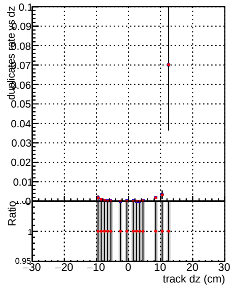
—●— DQM_V0001_R000000001 Global CMSSW_orig —●— DQM_V0001_R000000001 Global mkFitALLCHA RECO
