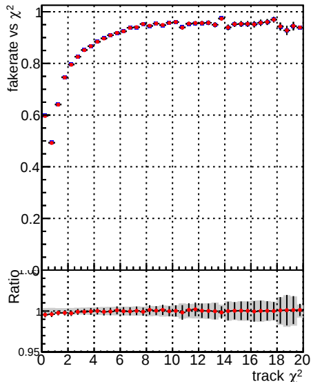
Fake rate vs. DQM_V0001_R000000001 Global CMSSW_orig DQM_V0001_R000000001 Global mkFitALLCHA
