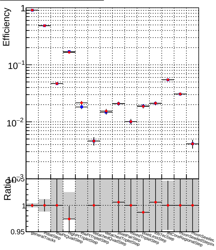
DQM_V0001_R000000001_Global_CMSSW_orig DQM_V0001_R000000001_Global_mkFitALLCHA_RECO
