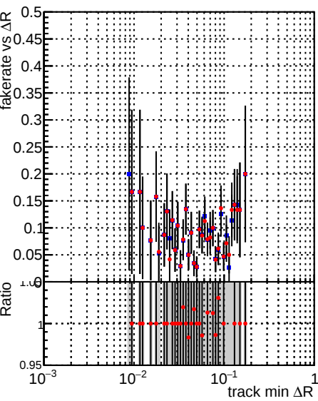
Fake rate vs \Delta R(\text{track, jet}) Legend: DQM_V0001_R000000001_Global_CMSSW_orig DQM_V0001_R000000001_Global_mkFitALLCHA_RECO
