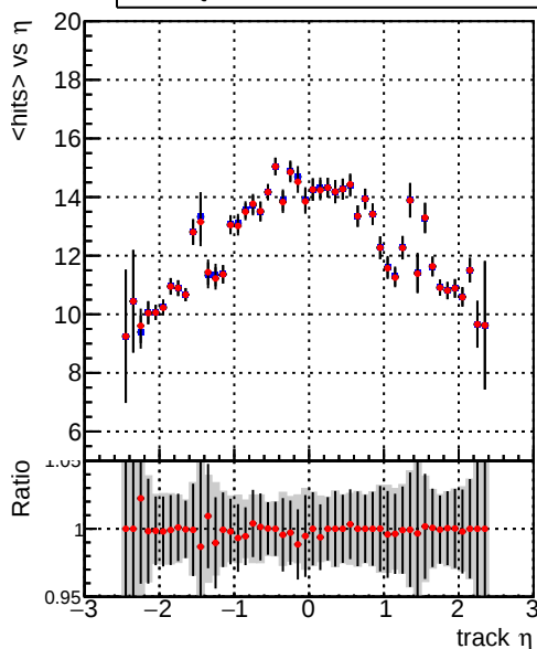
— DQM_V0001_R000000001_Global_CMSSW_orig — DQM_V0001_R000000001_Global_mkFitALLCHA_RECO
