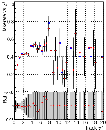
Fake rate vs. DQM V0001_R000000001 Global CMSSW_orig DQM V0001_R000000001 Global mkFitALLCHA DQM V0001_R000000001 Global RECO
