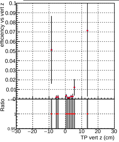
Efficiency vs vertpos Legend: DQM_V0001_R000000001_Global_mkFit100_RECO DQM_V0001_R000000001_Global_mkFitALLCHAI100_RECO
