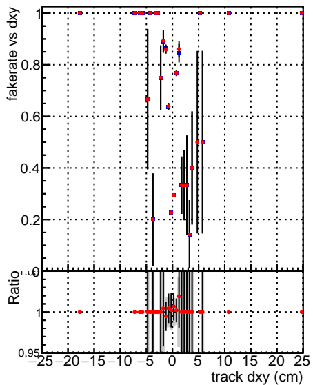
█ ● DQM_V0001_R000000001_Global_mkFit100_RECO █ ● DQM_V0001_R000000001_Global_mkFitALLCHAI100_RECO
