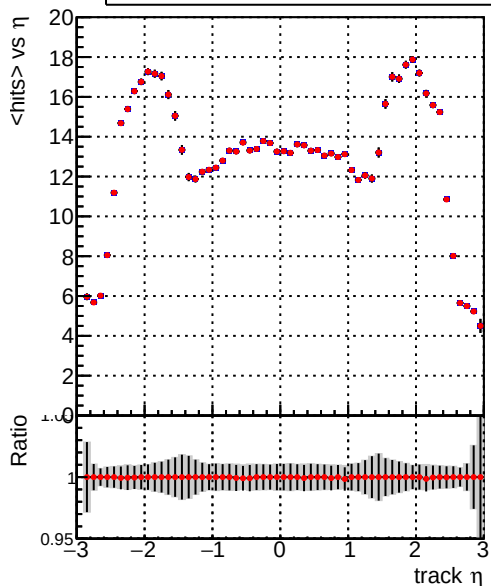
mean hit — DQM_V0001_R000000001_Global_mkFit100_RECO — DQM_V0001_R000000001_Global_mkFitALLCHAI100_RECO
