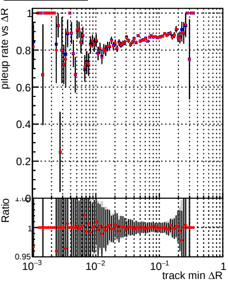
Legend: \blacksquare DQM_V0001_R000000001_Global_mkFit100_RECO \bullet DQM_V0001_R000000001_Global_mkFitALLCHAI100_RECO
