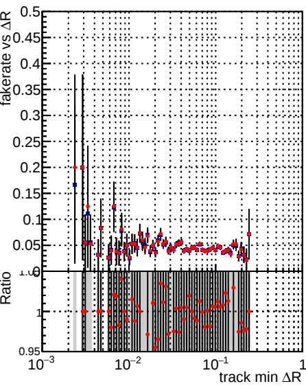
Legend: \blacksquare DQM_V0001_R000000001_Global_mkFit100_RECO \bullet DQM_V0001_R000000001_Global_mkFitALLCHAI100_RECO
