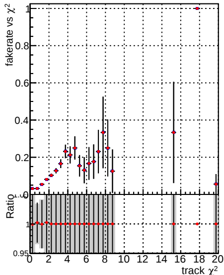
Fake rate vs. —●— DQM_V0001_R0000000001_Global_mkFit100_RECO —●— DQM_V0001_R0000000001_Global_mkFitALLCHAI100_RECO
