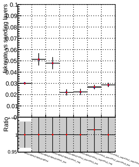
Fake rate vs. —•— DQM_V0001_R000000001_Global_mkFit100_RECO —•— DQM_V0001_R000000001_Global_mkFitALLCHAI100_RECO
