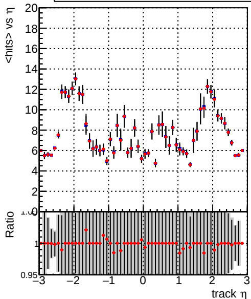
— DQM_V0001_R000000001_Global_mkFit100_RECO — DQM_V0001_R000000001_Global_mkFitALLCHAI100_RECO
