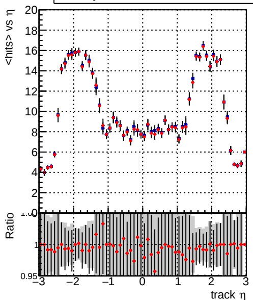
— DQM_V0001_R000000001_Global_mkJFit100_RECO — DQM_V0001_R000000001_Global_mkJFitALLCHAI100_RECO
