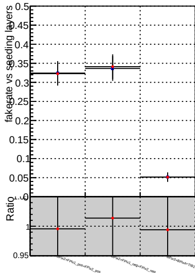
Fake rate vs. —•— DQM V0001_R000000001 Global mkFit100 RECO —•— DQM V0001_R000000001 Global mkFitALLCHAI100 RECO
