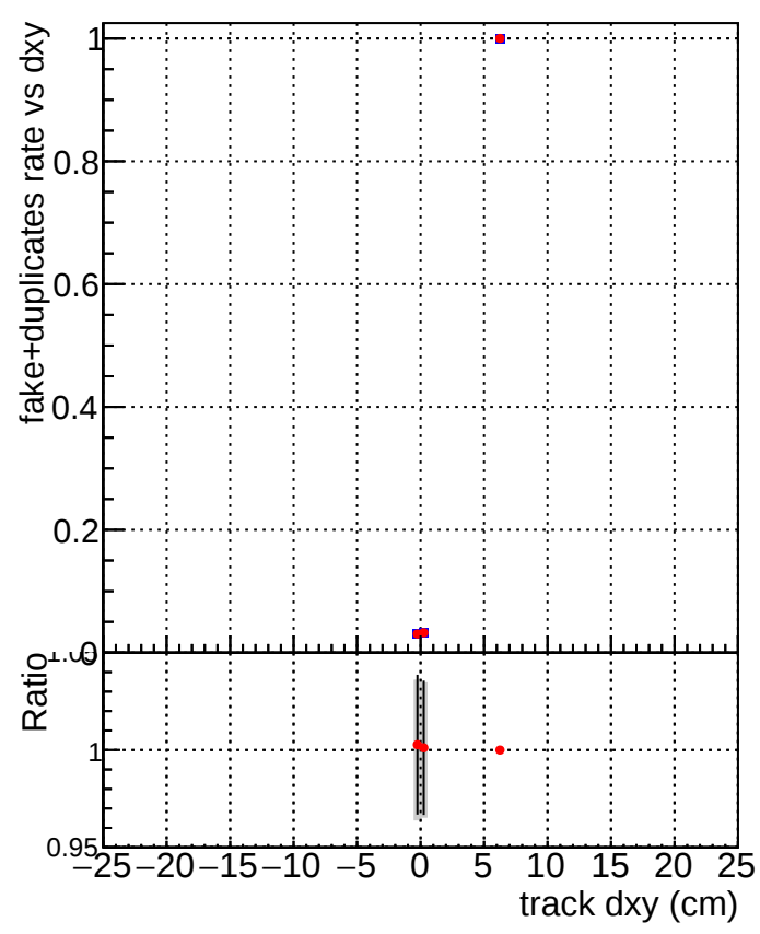
DQM_V0001_R000000001_Global_mkFit100_RECO DQM_V0001_R000000001_Global_mkFitALLCHAI100_RECO
