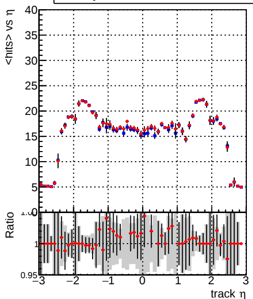
mean hits vs \eta — DQM_V0001_R000000001_Global_mkFit100_RECO — DQM_V0001_R000000001_Global_mkFitALLCHAI100_RECO
