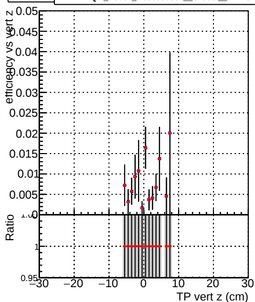
Efficiency vs. TP vert z —●— DQM_V0001_R000000001_Global_mkFit100_RECO —●— DQM_V0001_R000000001_Global_mkFitALLCHAI100_RECO
