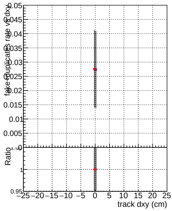
DQM_V0001_R000000001_Global_mkFitALLCHAI100_RECO
