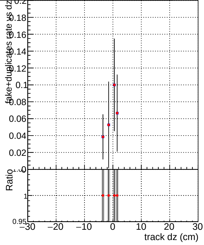
DQM_V0001_R000000001_Global_mkFitALLCHAI100_RECO
