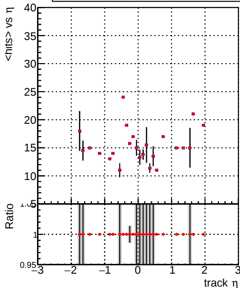
— DQM_V0001_R000000001_Global_mkFit100_RECO — DQM_V0001_R000000001_Global_mkFitALLCHAI100_RECO
