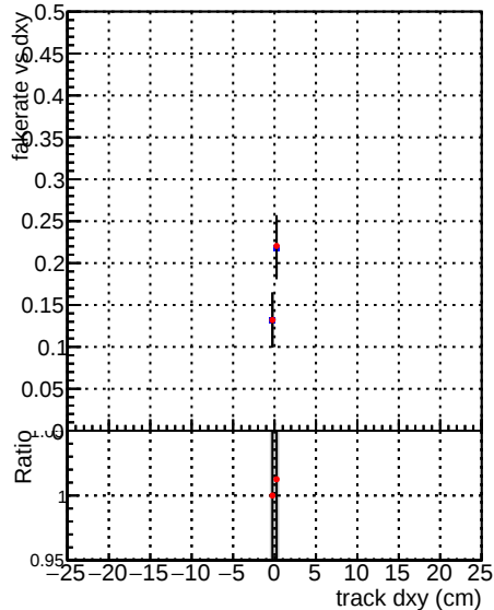
—●— DQM_V0001_R0000000001_Global_mkFit100_RECO —●— DQM_V0001_R0000000001_Global_mkFitALLCHAI100_RECO
